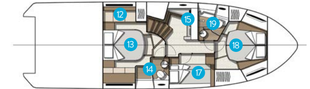
GT46 LOWER DECK - 3 CABINS
